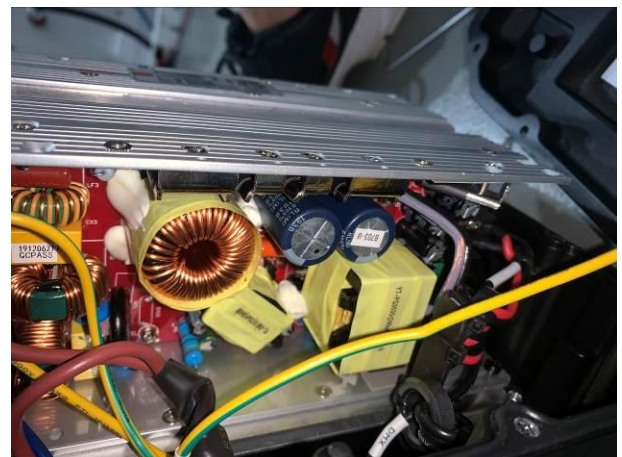
Photo 12 After the waterproof test, no water entry into internal.
