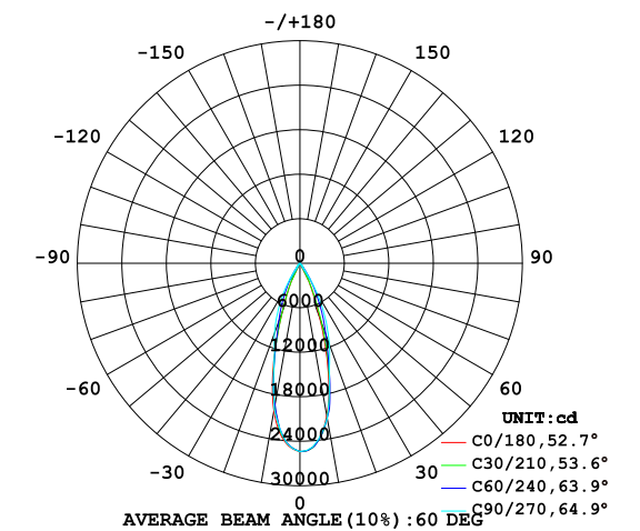
LUMINOUS INTENSITY DISTRIBUTION DIAGRAM
